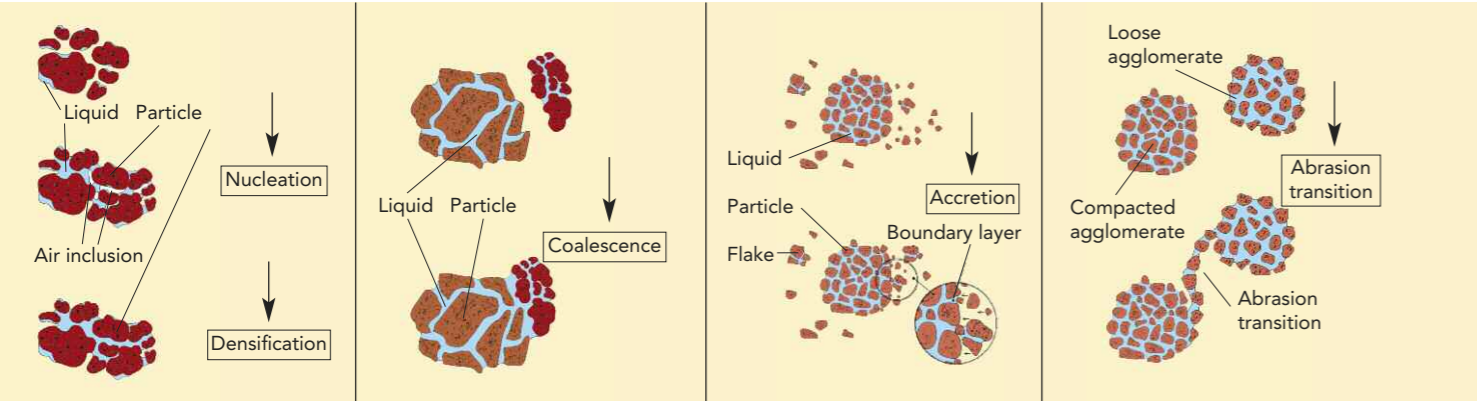
Principle of agglomeration
